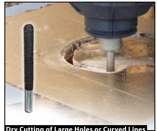
Dry Cutting of Large Holes or Curved Lines VACUUM BRAZED TRIMMER BIT
