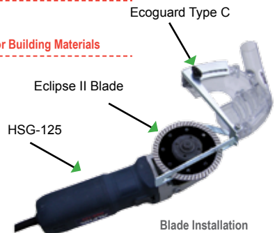
HSG-125 attached to Ecoguard Type C
